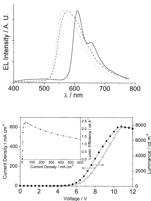
Fig. 21 Top: normalized electroluminescence spectra for (dotted line) 30 , (dashed line) [Pt(C 1 N 1 N 1 N)(C≡CC 6 H 4 Me-4)], and (continuous line) 40 at 4% doping level and multi-layer configuration of device. Bottom: current density, voltage and luminance characteristics (inset: luminescent efficiency vs current density) for OLED using 30 as emitter as 4% doping level (Reproduced with permission from [36a]. Copyright 2002 Royal Society of Chemistry)
