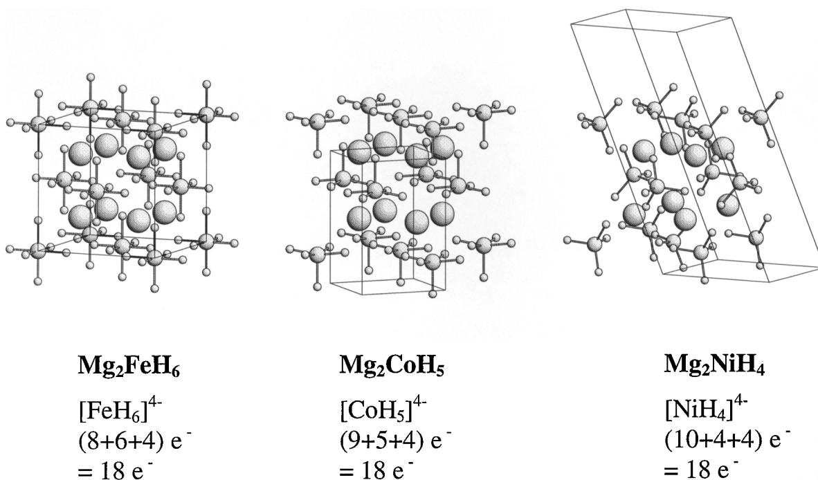
FIGURE 6 Crystal structures of cubic Mg 2 FeH 6 (K 2 PtCl 6 type), tetragonal Mg 2 CoH 5 , and monoclinic Mg 2 NiH 4 . Large spheres represent Mg, middle-sized spheres the transition metal M (Fe, Co, Ni), and small spheres H. M–H bonds in the transition metal hydrido complexes are drawn out. For Mg 2 NiH 4 , an incomplete unit cell is shown. Note the close resemblance of the geometrical arrangements of Mg cations and transition metal complex anions in all three structures.
