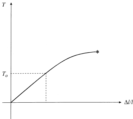
Fig. 1.3.3.2. Schematic stress-strain curve. T : stress; T_o : elastic limit; \Delta l/l : elongation; the asterisk symbolizes the rupture.
