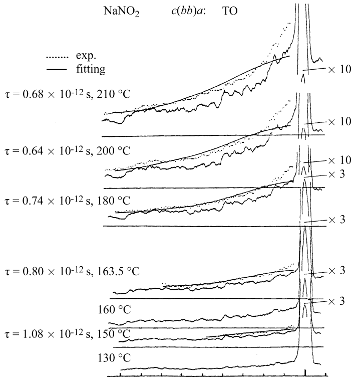
Fig. 3.1.5.20. Raman spectra of sodium nitrite, showing diffusive Debye-like response due to large-amplitude flopping over of nitrite ions [note that the high-frequency phonon-like response is due to the small-amplitude motion of this same normal mode; thus in this system N ions give rise not to 3N (non-degenerate) peaks in the spectral response function, but to 3N + 1 ].
