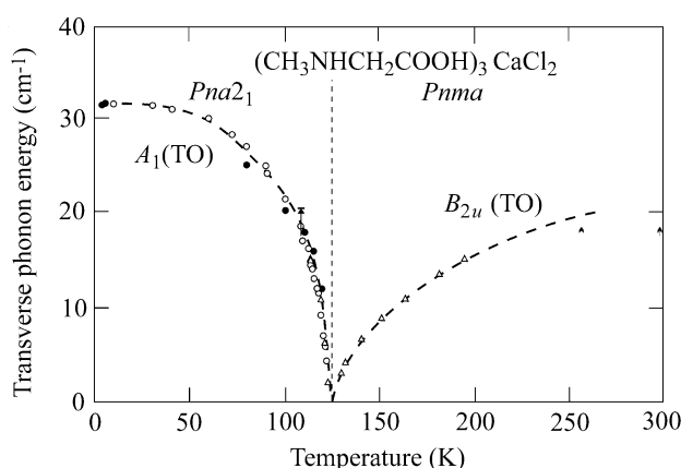
Fig. 3.1.5.15. 'Soft' optical phonon frequencies versus temperature in both ferroelectric and paraelectric phases of tris-sarcosine calcium chloride.
