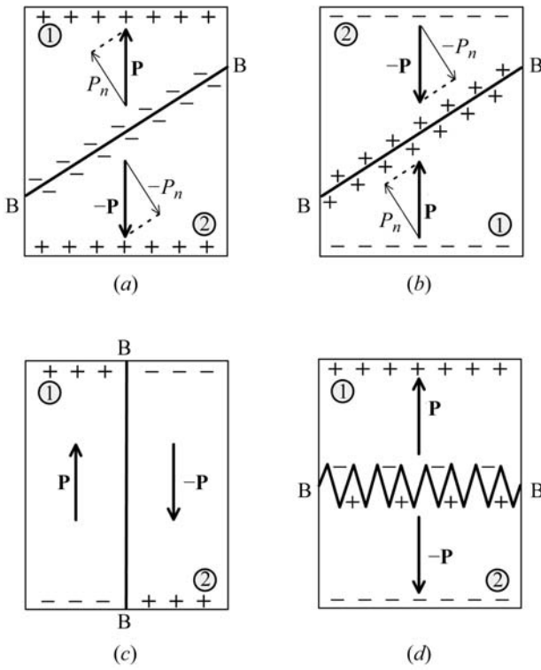
Fig. 3.3.10.2. Boundaries B-B between 180° domains (merohedral twins) of pyroelectric crystals. (a) Tail-to-tail boundary. (b) Head-to-head boundary. (c) Uncharged boundary ( P_n = 0 ). (d) Charged zigzag boundary, with average orientation normal to the polar axis. The charge density is significantly reduced. Note that the charges at the boundaries are usually compensated by stray charges of opposite sign.
